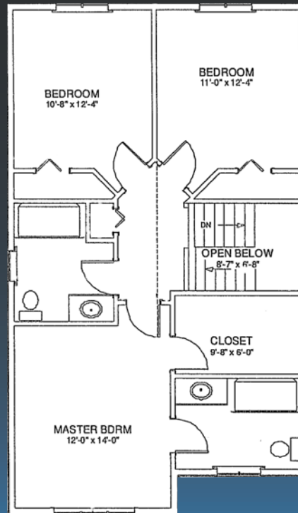
Second Floor 876 sq.ft.
